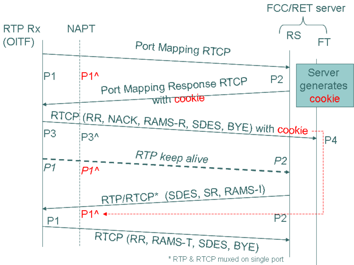
Figure 13: NATP traversal for FCC/RET with cookie signaling
