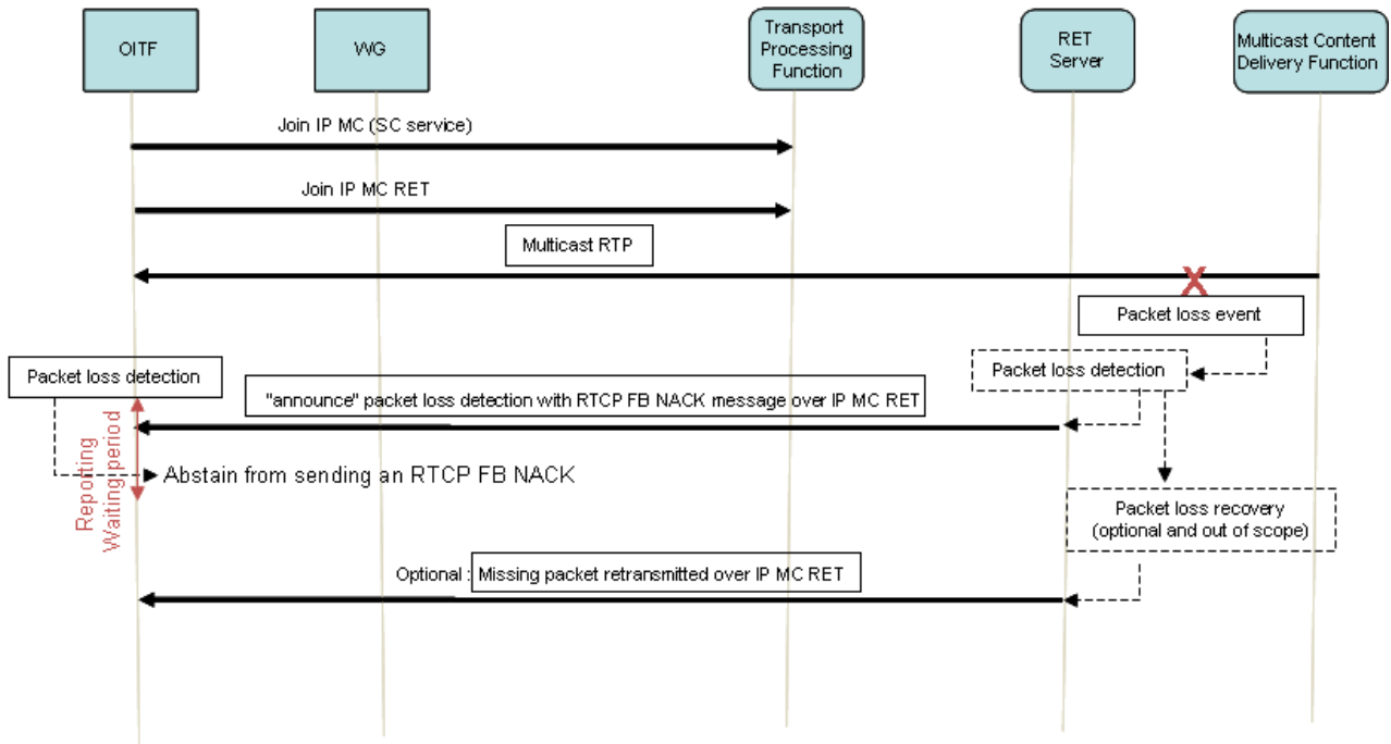
Figure 18: MC RET protocol interaction for packet loss upstream of RET server
