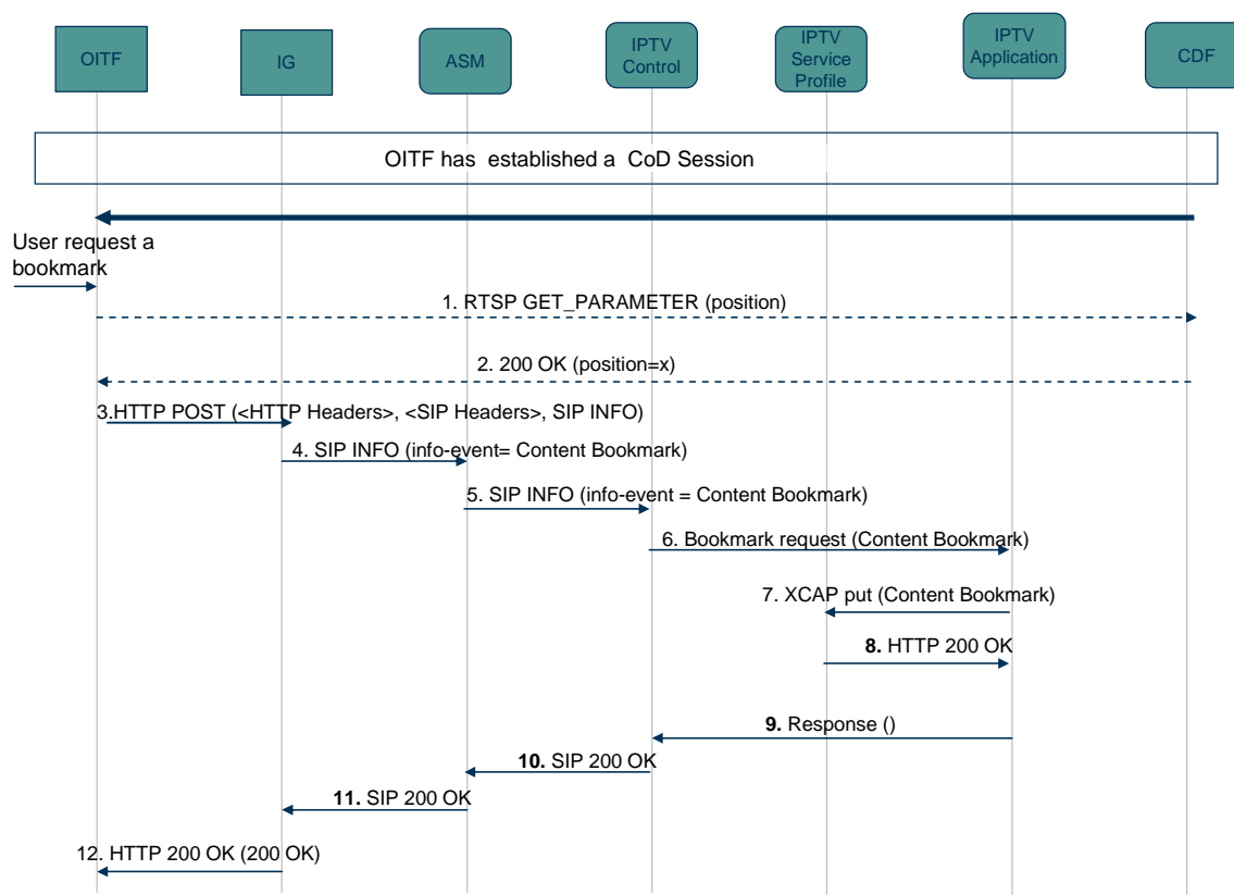
Figure 23: Content Bookmarking in a Content on Demand Session
