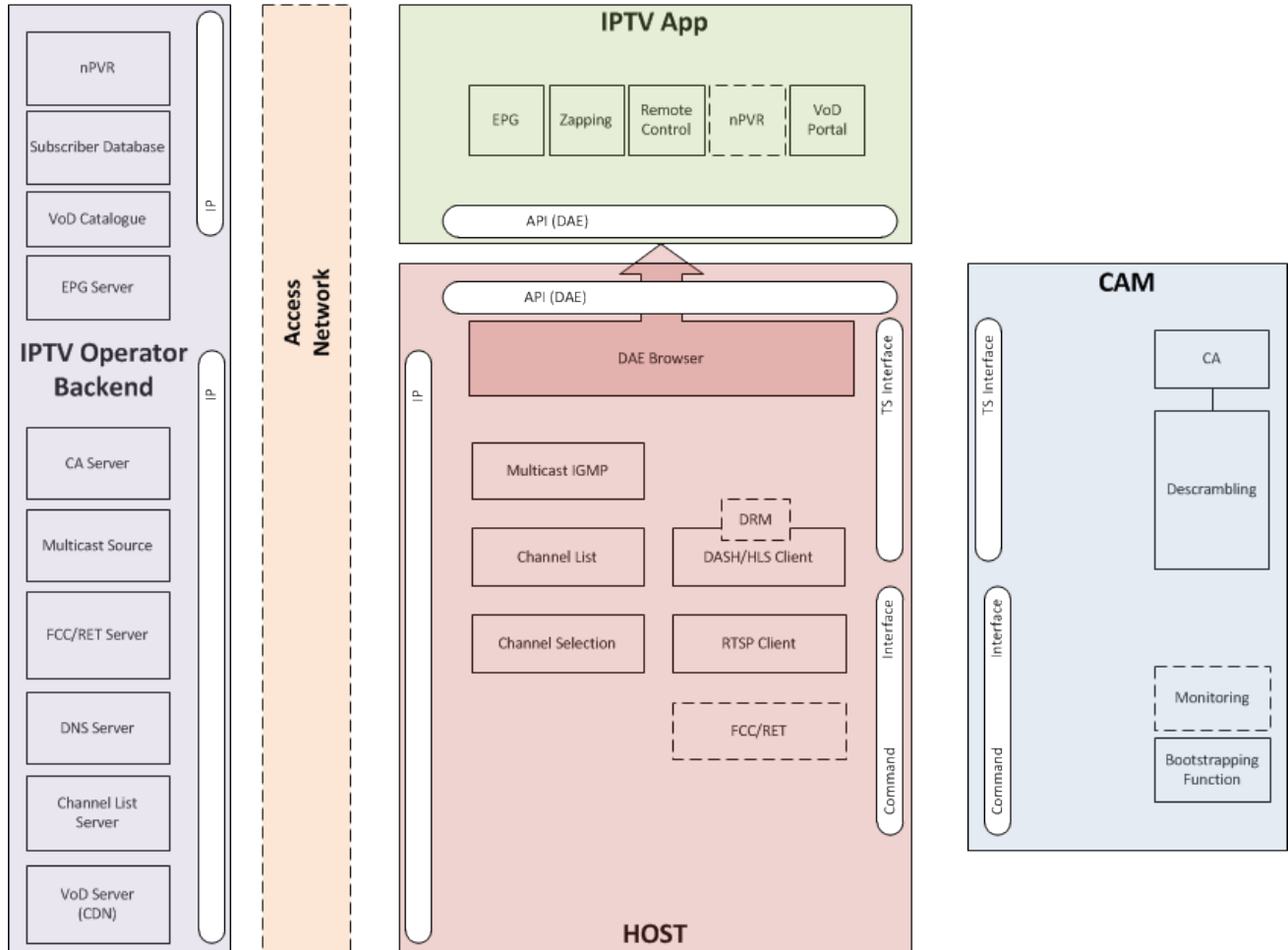
Figure 1: High-level block diagram including the major components making up the CAM-based STB-less IPTV System
